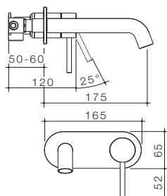
LIANO II 175MM WALL BASIN/BATH MIXER - ROUND COVER PLATE
