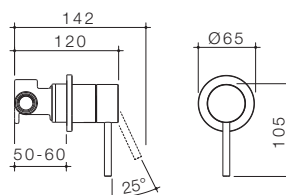
LIANO II BATH/SHOWER MIXER - ROUND COVER PLATE
