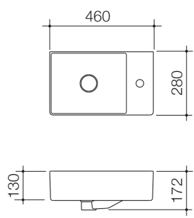
URBANE II HAND WALL BASIN
