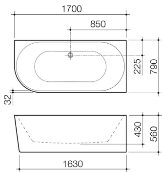
URBANE II BACK TO CORNER 1700 BATH RIGHT HAND SIDE NO OVERFLOW UII7RHCW
