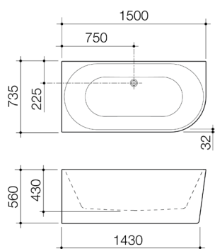
URBANE II BACK TO CORNER 1500 BATH LEFT HAND SIDE NO OVERFLOW UII5LHCW
