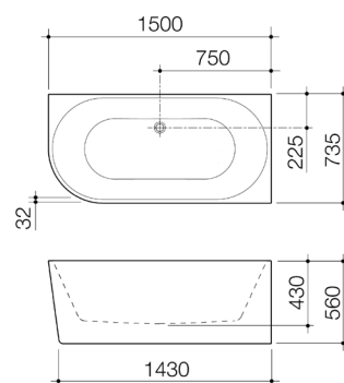
URBANE II BACK TO CORNER 1500 BATH RIGHT HAND SIDE NO OVERFLOW UII5RHCW
