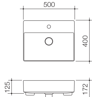
URBANE II SEMI RECESSED BASIN
