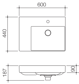
URBANE II LEFT HAND SHELF WALL BASIN
