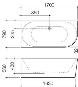
URBANE II BACK TO CORNER 1700 BATH LEFT HAND SIDE NO OVERFLOW UII7LHCW
