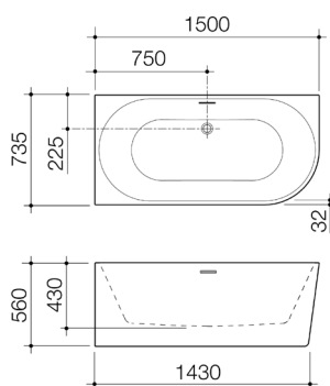
URBANE II BACK TO CORNER 1500 BATH LEFT HAND SIDE OVERFLOW UII5LHCWOF
