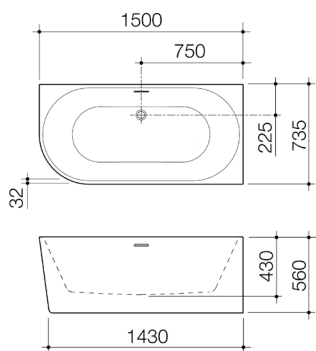
URBANE II BACK TO CORNER 1500 BATH RIGHT HAND SIDE OVERFLOW UII5RHCWOF
