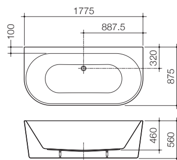
URBANE II 1800 BACK TO WALL FREESTANDING BATH AU8WFW
