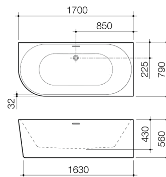
URBANE II BACK TO CORNER 1700 BATH RIGHT HAND SIDE OVERFLOW OF UII7RHCW
