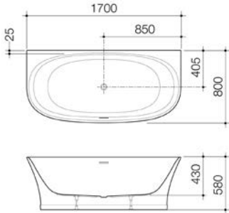
CAROMA RIVIERE 1700MM FREESTANDING BATH WITH OVERFLOW Matte White EN7FSMWOF White EN7FSWOF
