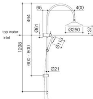
CAROMA RIVIERE RAIL SHOWER WITH OVERHEAD
