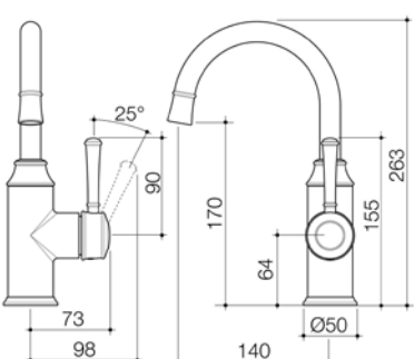
CAROMA RIVIERE GOOSENECK BASIN MIXER Chrome Brushed Bronze 520004C6AF 520004BBZ6AF Brushed Brass Brushed Nickel 520004BB6AF 520004BN6AF
