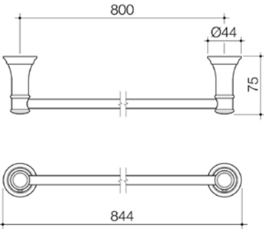
CAROMA RIVIERE SINGLE TOWEL RAIL 800MM
