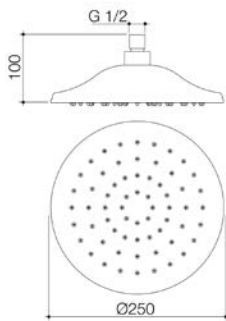
CAROMA RIVIERE RAIN SHOWER 250MM
