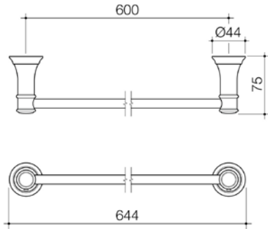
CAROMA RIVIERE SINGLE TOWEL RAIL 600MM Chrome 520034C Brushed Bronze 520034BBZ Brushed Brass 520034BB Brushed Nickel 520034BN
