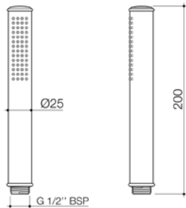
CAROMA RIVIERE MICROPHONE HANDSET
