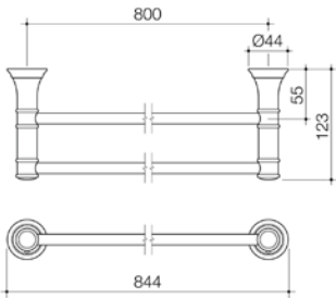
CAROMA RIVIERE DOUBLE TOWEL RAIL 800MM
