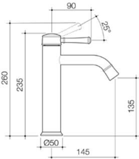
CAROMA RIVIERE MID TOWER BASIN MIXER Chrome Brushed Bronze 520002C6AF 520002BBZ6AF Brushed Brass Brushed Nickel 520002BB6AF 520002BN6AF
