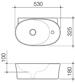
CAROMA RIVIERE HAND WALL BASIN - 1 TAP HOLE Matte White 4700510MW White 4700510W
