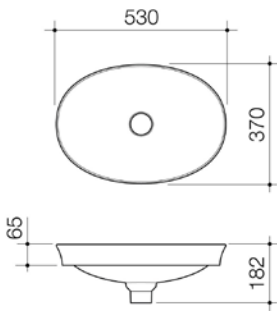
CAROMA RIVIERE 530MM INSET BASIN NO TAP HOLE White 4700100W Matte White 4700100MW
