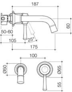
CAROMA RIVIERE WALL BASIN/BATH MIXER 175MM Chrome Brushed Bronze 520009C6AF 520009BBZ6AF Brushed Brass Brushed Nickel 520009BB6AF 520009BN6AF
