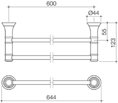
CAROMA RIVIERE DOUBLE TOWEL RAIL 600MM
