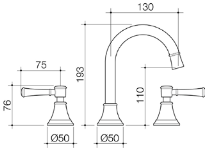
CAROMA RIVIERE HOB BASIN SET Chrome Brushed Bronze 520020C6AF 520020BBZ6AF Brushed Brass Brushed Nickel 520020BB6AF 520020BN6AF
