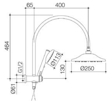
CAROMA RIVIERE COMPACT TWIN SHOWER
