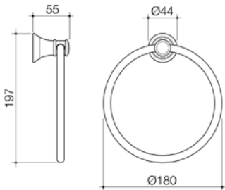
CAROMA RIVIERE TOWEL RING Chrome 520032C Brushed Bronze 520032BBZ Brushed Brass 520032BB Brushed Nickel 520032BN
