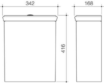
RIVIERE CLOSE COUPLED BACK ENTRY CISTERN
