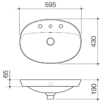
CAROMA RIVIERE 595MM INSET BASIN WITH 3 TAP HOLE Overflow feature No overflow feature Matte White Matte White 4700235MW 4700230MW White White 4700235W 4700230W
