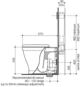
CAROMA RIVIERE CLEANFLUSH® INVISI SERIES II® WALL FACED SUITE WITH GERMGARD®
