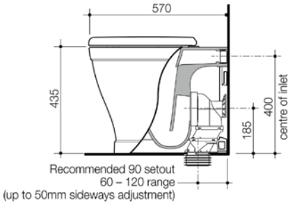
RIVIERE CLEANFLUSH® WALL FACED BOTTOM INLET PAN
