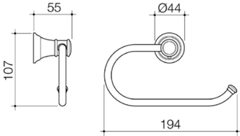
CAROMA RIVIERE TOILET ROLL HOLDER Chrome 520030C Brushed Bronze 520030BBZ Brushed Brass 520030BB Brushed Nickel 520030BN
