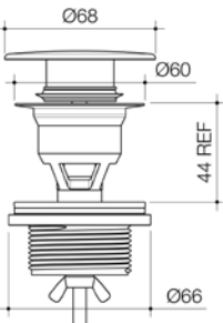
CAROMA BASIN DOME POP UP WASTE
