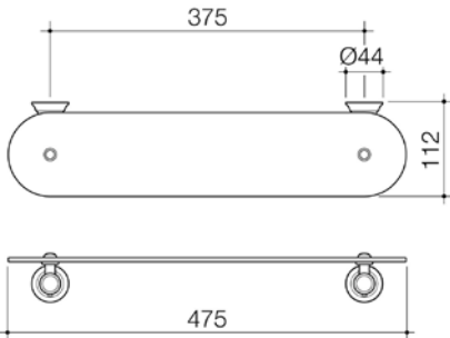
CAROMA RIVIERE BATHROOM SHELF Chrome 520038C Brushed Bronze 520038BBZ Brushed Brass 520038BB Brushed Nickel 520038BN
