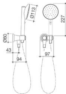
CAROMA RIVIERE VJET HAND SHOWER
