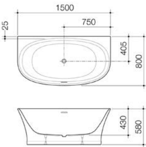
CAROMA RIVIERE 1500MM BACK TO WALL FREESTANDING BATH WITH OVERFLOW FEATURE Matte White EN5WFMWOF White EN5WFWOF
