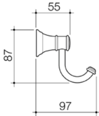
CAROMA RIVIERE ROBE HOOK Chrome 520031C Brushed Bronze 520031BBZ Brushed Brass 520031BB Brushed Nickel 520031BN
