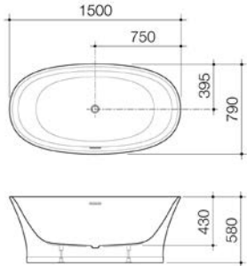
CAROMA RIVIERE 1500MM FREESTANDING BATH WITH OVERFLOW Matte White EN5FSMWOF White EN5FSWOF
