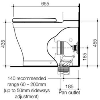
RIVIERE CLEANFLUSH® WALL FACED CLOSE COUPLED BOTTOM INLET PAN
