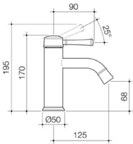
CAROMA RIVIERE BASIN MIXER Chrome Brushed Bronze 520001C6AF 520001BBZ6AF Brushed Brass Brushed Nickel 520001BB6AF 520001BN6AF
