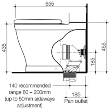
RIVIERE CLEANFLUSH® WALL FACED CLOSE COUPLED BACK ENTRY PAN
