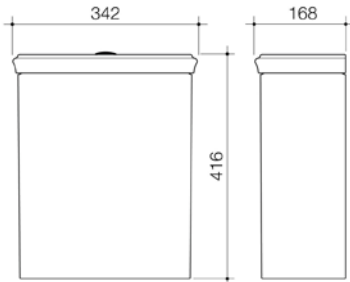
RIVIERE CLOSE COUPLED RIGHT HAND CISTERN
