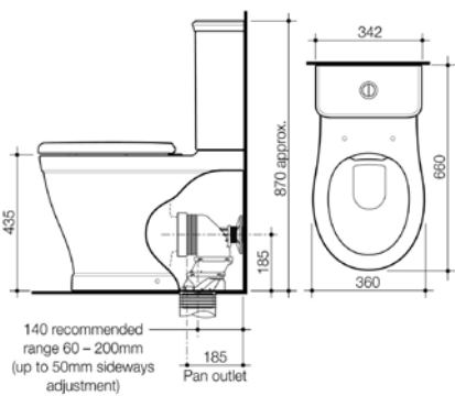
RIVIERE CLEANFLUSH® WALL FACED CLOSE COUPLED TOILET SUITE WITH GERMGARD®
