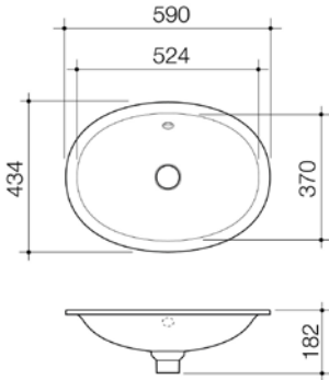
CAROMA RIVIERE UNDER COUNTER BASIN Overflow feature No Overflow feature Matte White Matte White 4700405MW 4700400MW White White 4700405W 4700400W
