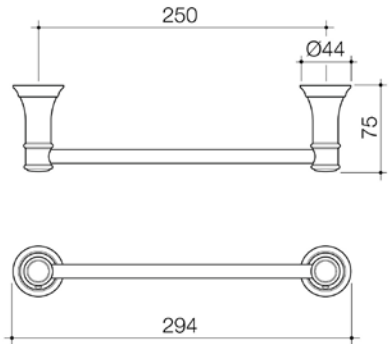
CAROMA RIVIERE HAND TOWEL RAIL Chrome 520033C Brushed Bronze 520033BBZ Brushed Brass 520033BB Brushed Nickel 520033BN
