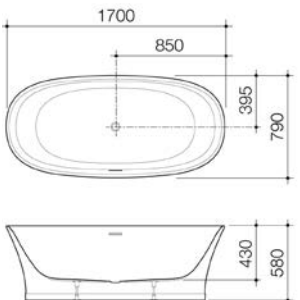
CAROMA RIVIERE 1700MM BACK TO WALL FREESTANDING BATH WITH OVERFLOW Matte White EN7WFMWOF White EN7WFWOF
