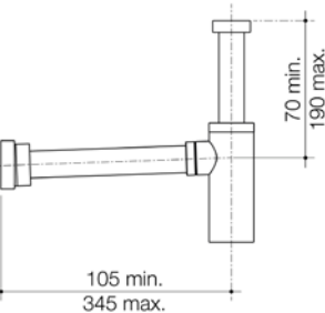
CAROMA 40MM BOTTLE TRAP
