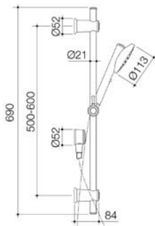
CAROMA RIVIERE RAIL SHOWER
